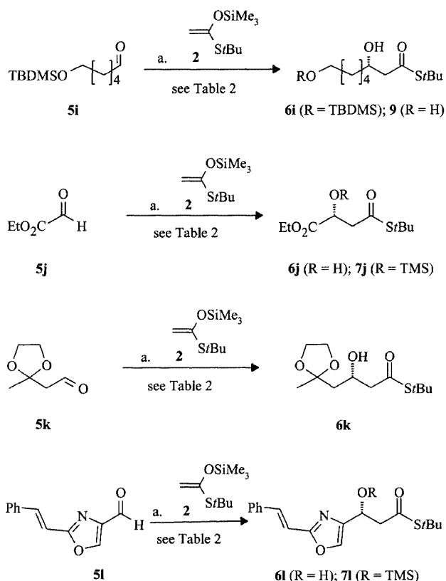
Scheme 4. a) ( R )-BINOL-Ti 4a , Et 2 O, (phenol), 0 °C, 5 h, then 0 °C to room temp., 16 h
